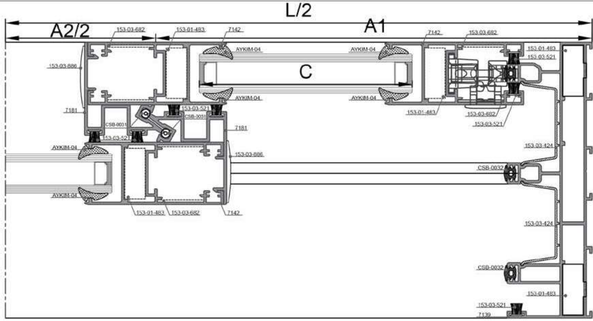
15-15 DETAYI DETAIL
