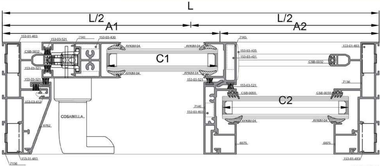
1-1 DETAYI DETAIL
