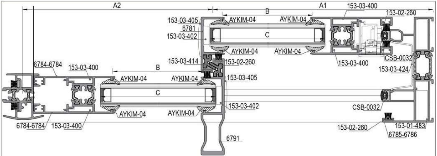
12-12 DETAYI 12-12 DETAIL
