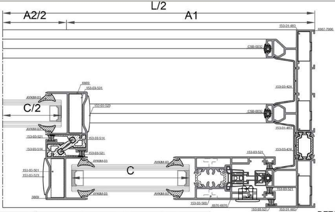
9-9 DETAYI DETAIL
