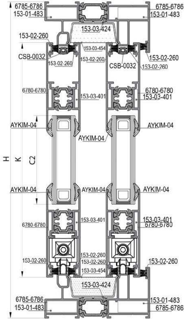
13-13 DETAYI 13-13 DETAIL
