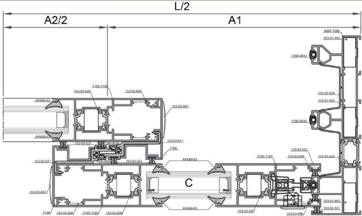
15-15 DETAYI DETAIL
