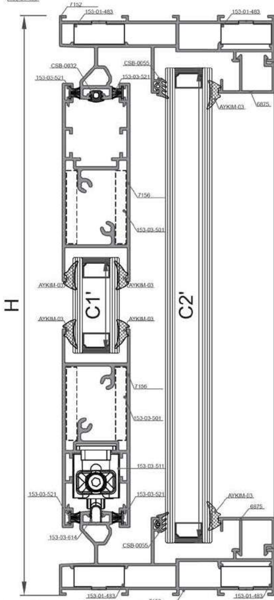
3-3 DETAYI DETAIL
