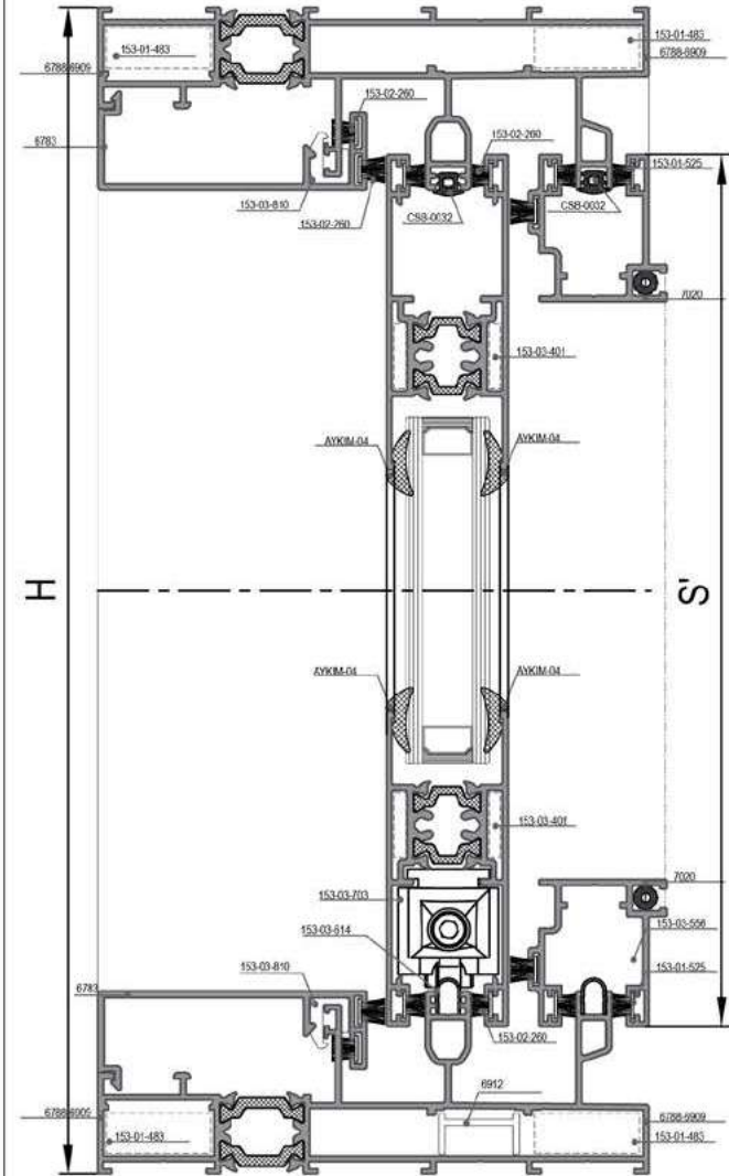
5-5 DETAYI 5-5 DETAIL
