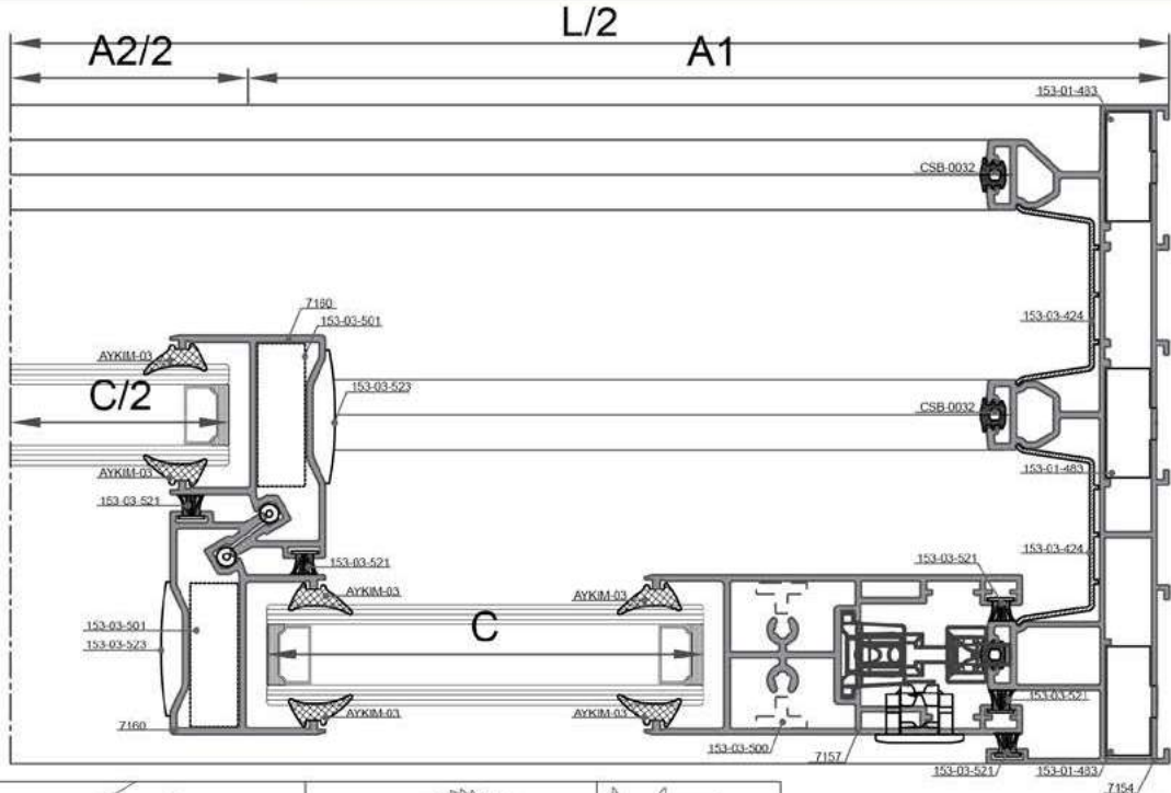
DETAYI 9-9 DETAIL
