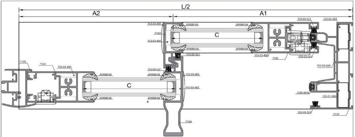
7-7 DETAYI DETAIL
