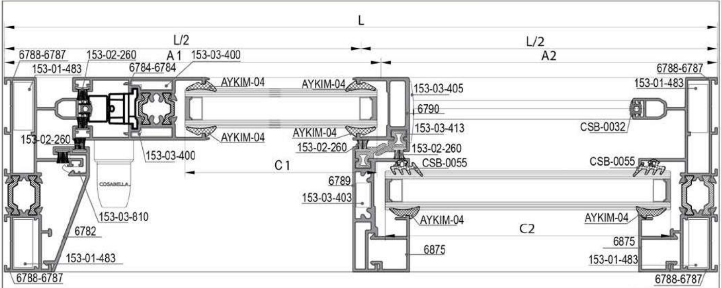
1-1 DETAYI 1-1 DETAIL
