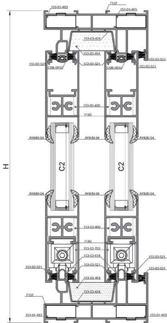
8-8 DETAYI DETAIL
