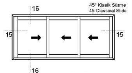
16-16 DETAYI DETAIL
