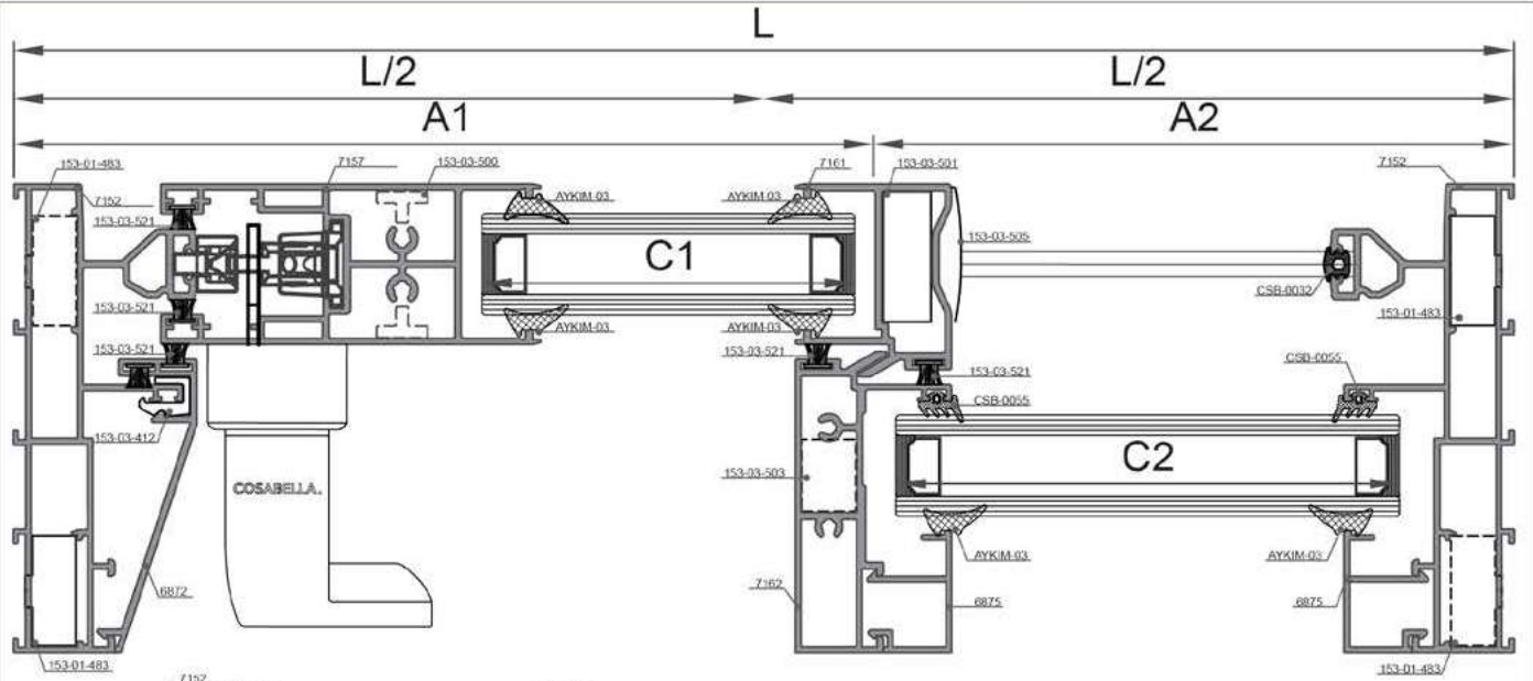
1-1 DETAYI DETAIL
