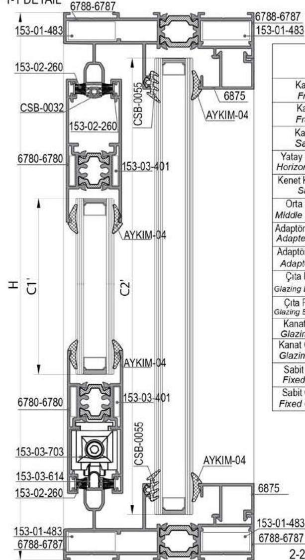
1-1 DETAYI 1-1 DETAIL
