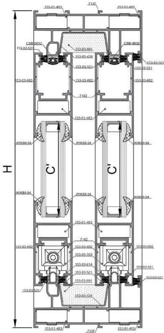
14-14 DETAYI DETAIL
