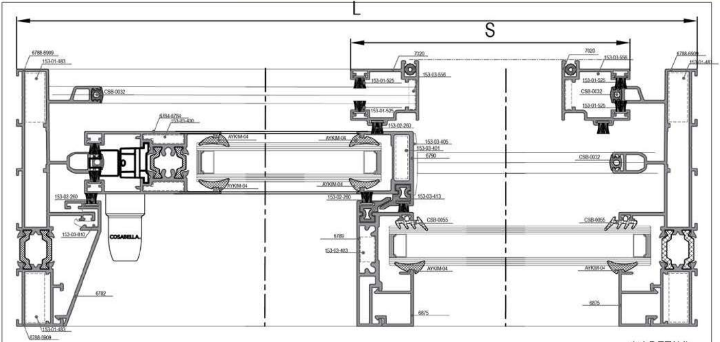
4-4 DETAYI 4-4 DETAIL
